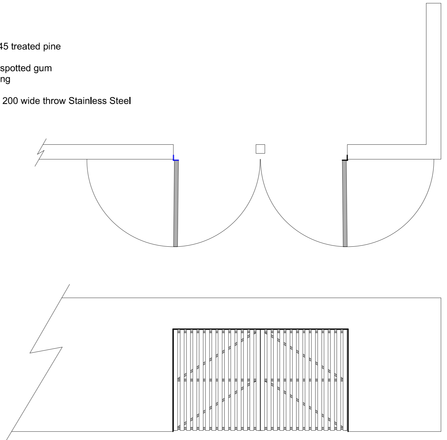
Double Doors Front Elevation
